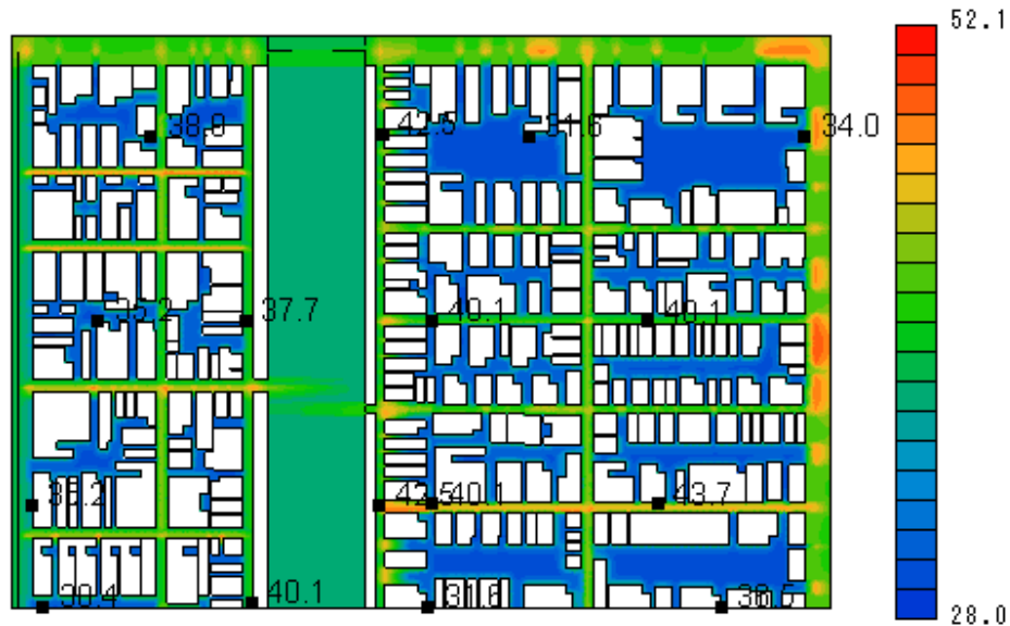
Figure 13 Air temperature distribution for Pattern F
