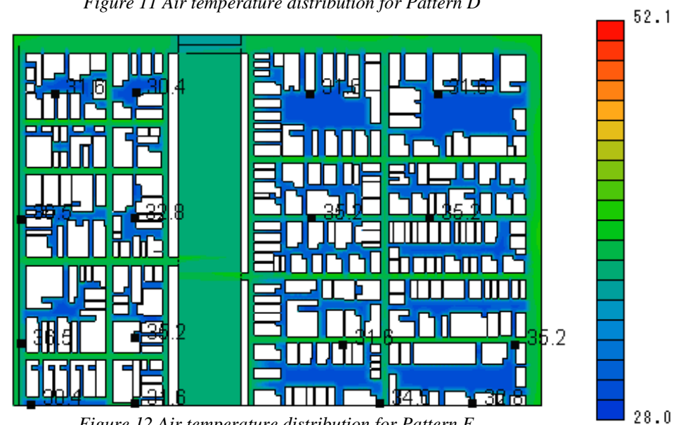
Figure 12 Air temperature distribution for Pattern E
