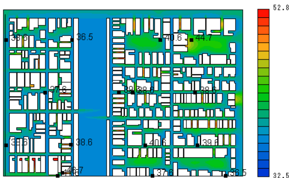
Figure 9 Air temperature distribution for Pattern B
