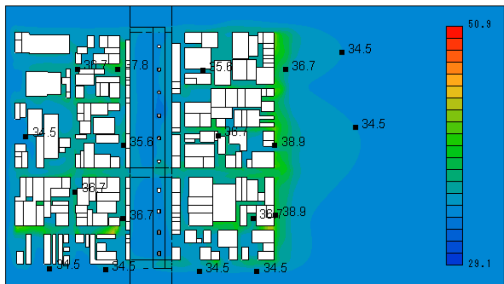
Figure 8 Air temperature distribution for Pattern A (Present town's configuration)
