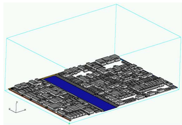
Figure 7 Model of Higashi-Yokobori District
