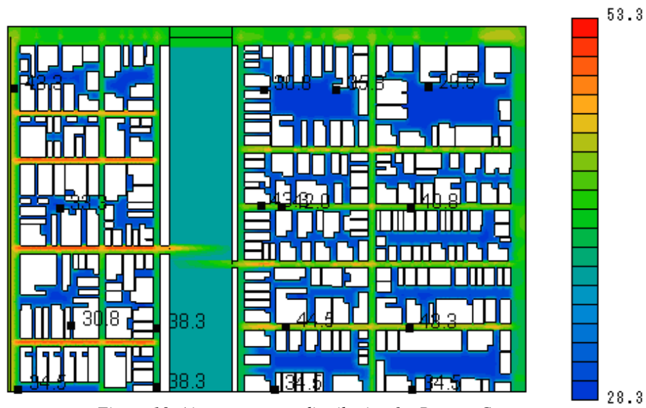
Figure 10 Air temperature distribution for Pattern C
