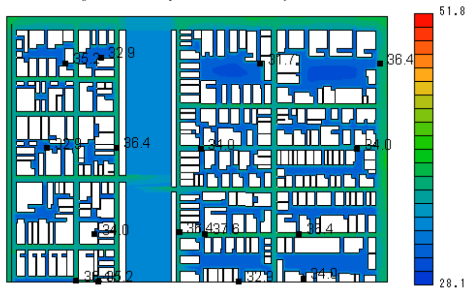
Figure 11 Air temperature distribution for Pattern D
